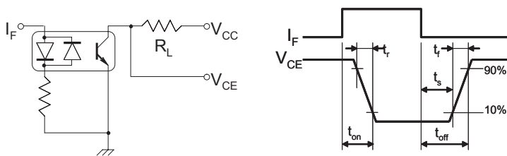
Figure 1. Switching Time Test Circuit
