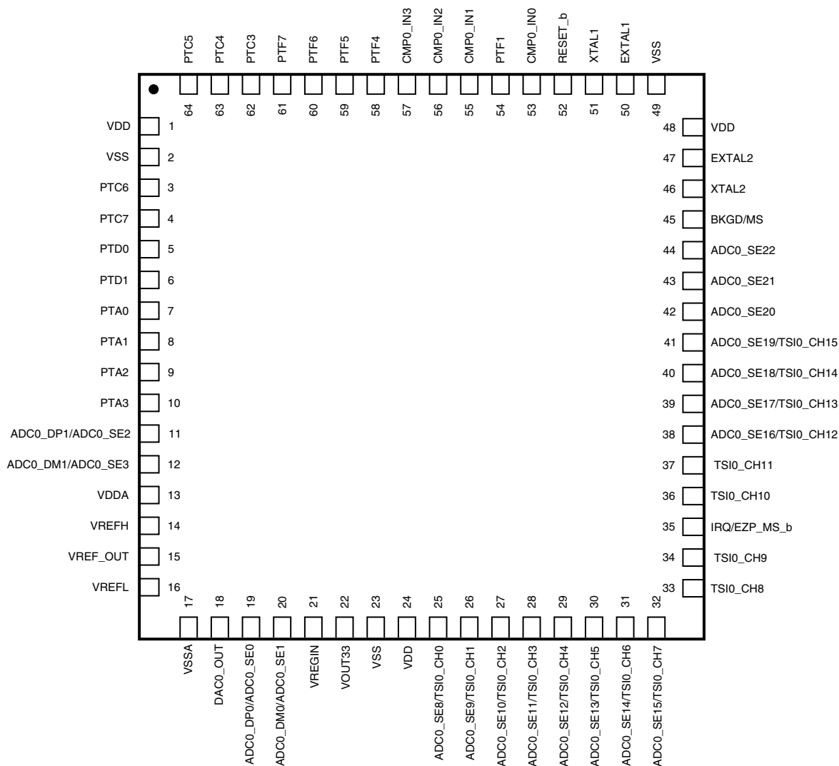
Figure 22. 64-pin Laminate QFN (pinout identical for 64-pin LQFP)
