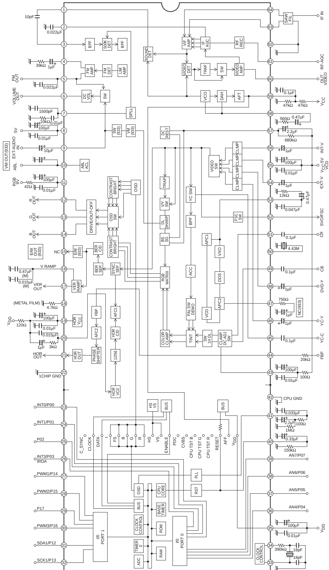
Block Diagram 1 LA76931J/933J
