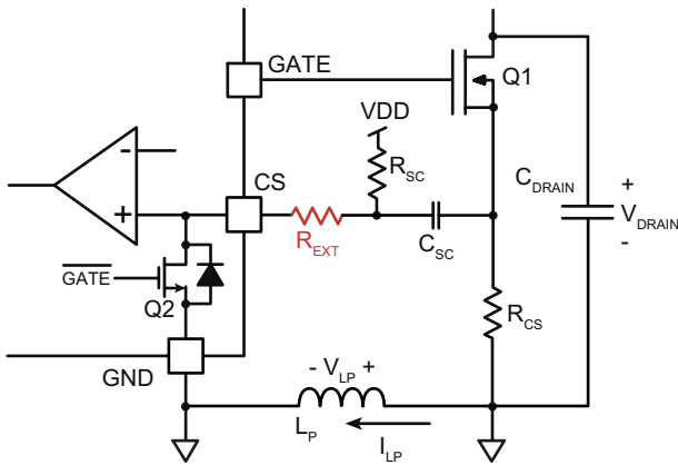
Fig. 4: Modified Slope Compensation Circuit
