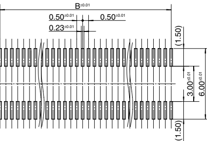
Recommended metal mask pattern Metal mask thickness: Here, 150 µm (Opening area ratio: 69%)
