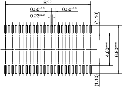
Recommended metal mask pattern Metal mask thickness: Here, 120 μm (Opening area ratio: 69%)
