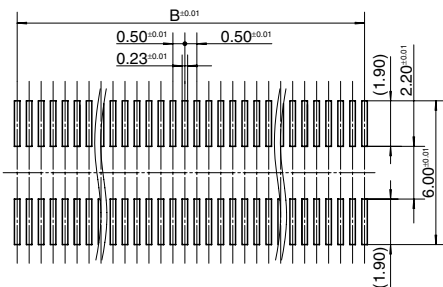
Recommended metal mask pattern Metal mask thickness: Here, 120 µm (Opening area ratio: 87%)
