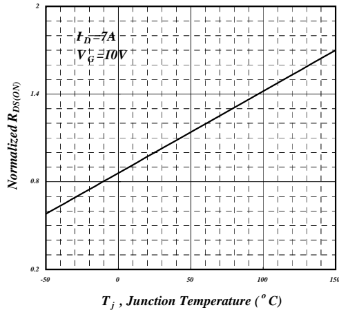
Fig 4. Normalized On-Resistance
