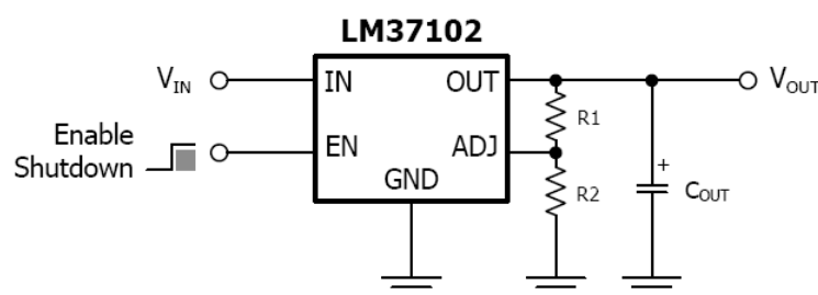
Figure 1. Adjustable Regulator with Resistors
