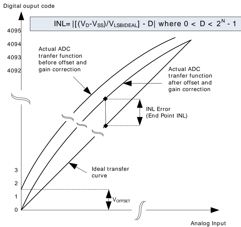
Figure 3.12. Integral Non-Linearity (INL)
