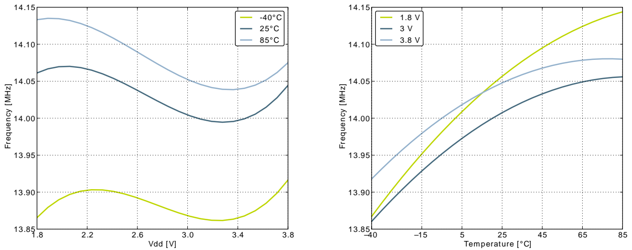
Figure 3.10. Calibrated HFRCO 21 MHz Band Frequency vs Temperature and Supply Voltage
