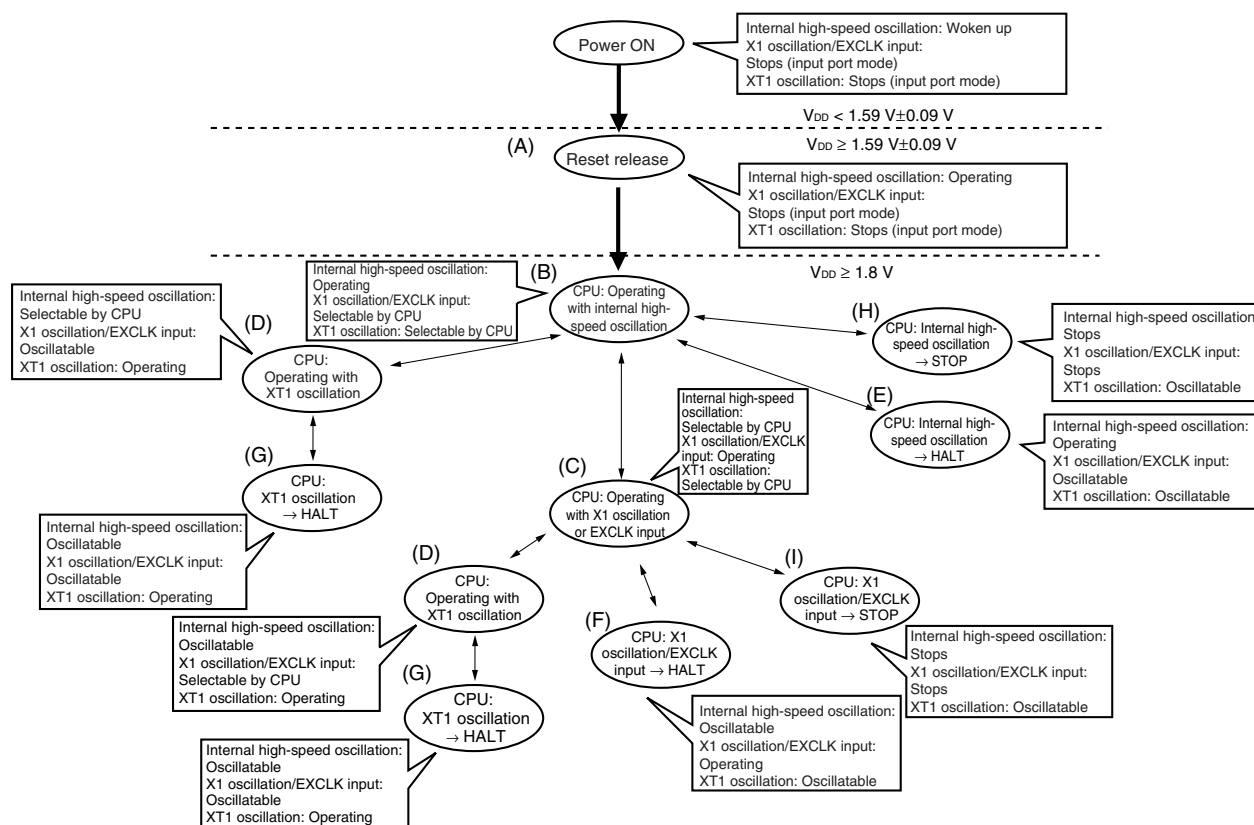
Figure 6-15. CPU Clock Status Transition Diagram
