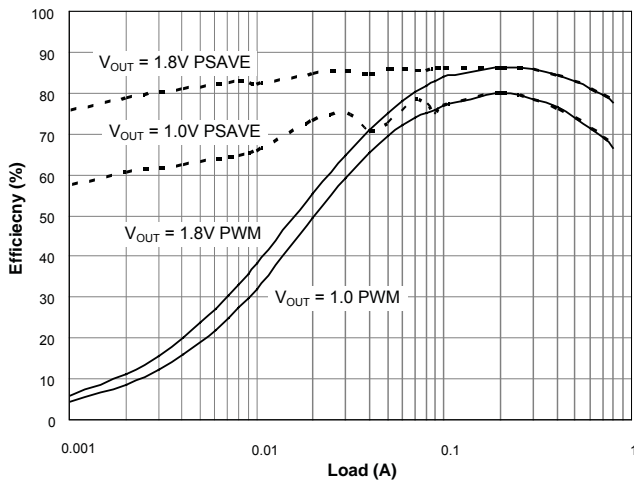
Efficiency vs. Load at V_{IN} = 5.5V , Side A
