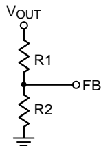
Figure 4. Setting V_{OUT} with a Resistive Voltage Divider
