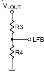
Figure 5. Setting V_{LOUT} with a Resistive Voltage Divider
