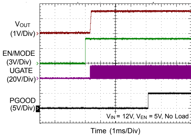
Power On from EN/MODE (CCM)
