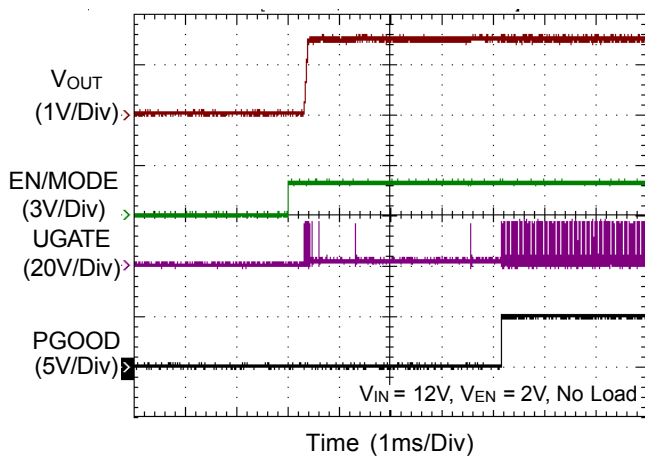
Power On from EN/MODE (USM)
