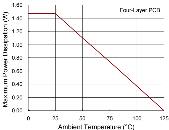
Figure 6. Derating Curve for the RT8234A Package
