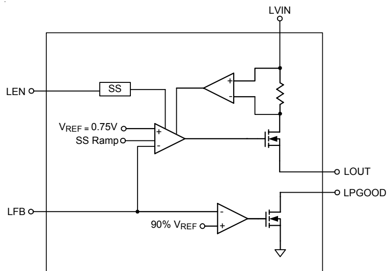
LDO Regulator
