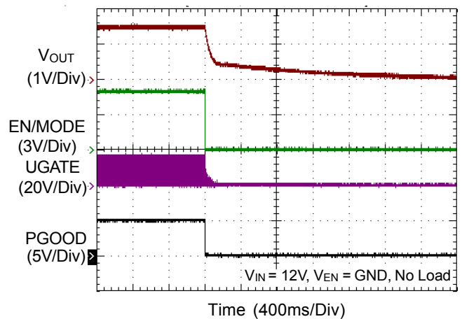
Power Off from EN/MODE (CCM)
