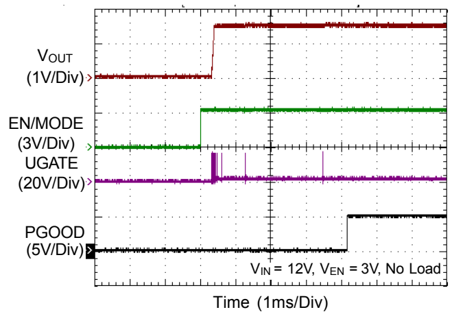
Power On from EN/MODE (DEM)
