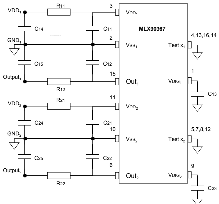
Figure 8 – Recommended wiring for the MLX90367 in TSSOP16 package (dual die)
