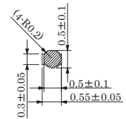
Recommended mounting hole (component-side view) *Please use 1.6mm thick PC board.
