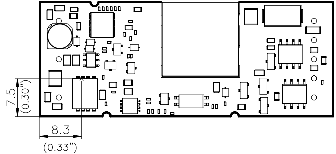
Figure 21: Hot spot temperature measured point The allowed maximum hot spot temperature is defined at 109°C
