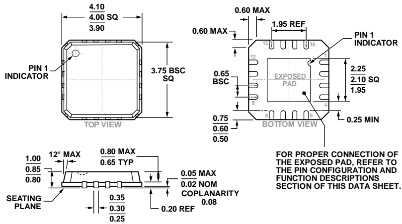
COMPLIANT TO JEDEC STANDARDS MO-220-VGGC Figure 49. 16-Lead Lead Frame Chip Scale Package [LFCSP_VQ] 4 mm × 4 mm Body, Very Thin Quad (CP-16-4) Dimensions shown in millimeters
