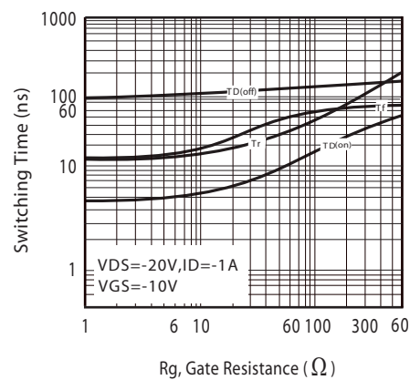
Figure 11. Switching Characteristics
