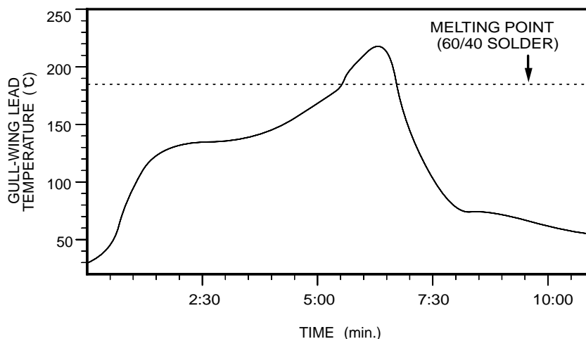
Figure 19. Typical Reflow Soldering Profile
