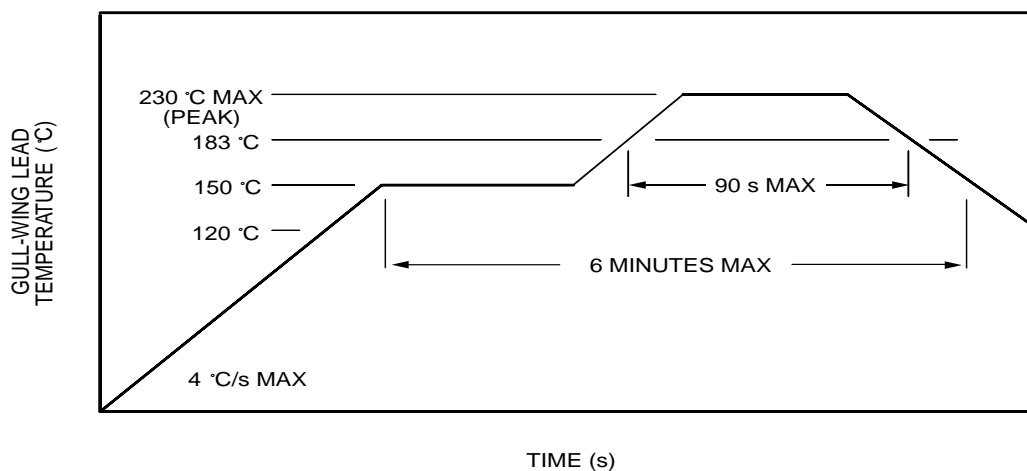
Figure 18. Maximum Thermal Profile Limits
