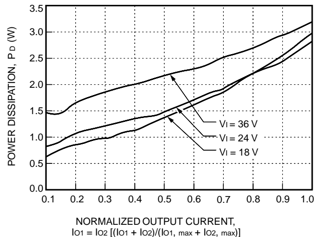
Figure 15. SMC010AJ, BK, CL Typical Power Dissipation vs. Normalized Output Current at T_c = 25^\circ\text{C}
