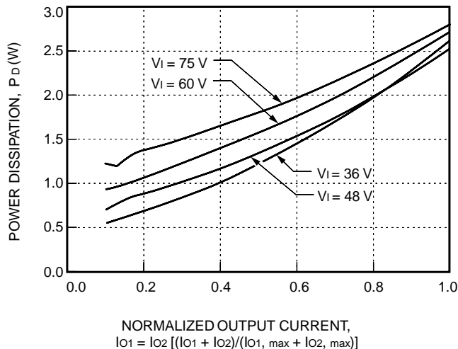
Figure 16. SMW010AJ, BK, CL Typical Power Dissipation vs. Normalized Output Current at T_c = 25^\circ\text{C}
