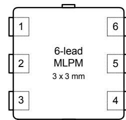
Figure 2. Package Type
