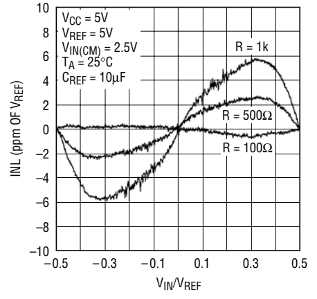
Figure 17. INL vs Differential Input Voltage and Reference Source Resistance for C REF > 1μF
