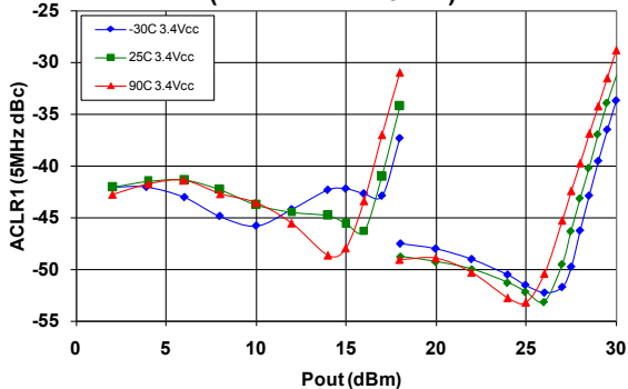
Figure 7: WCDMA ACLR1 (dBc) over Temperature ( V_{BATT} = V_{CC} = 3.4 V)
