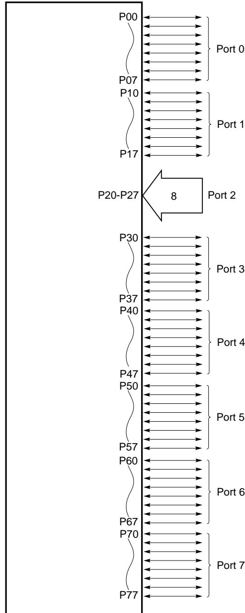
Figure 8-1. Port Configuration
