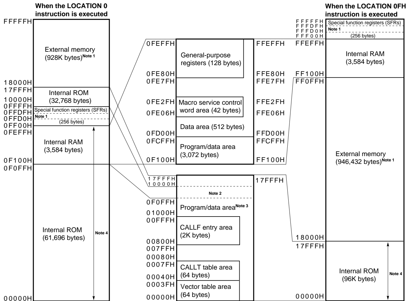
Figure 7-3. μPD784037 Memory Map
