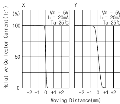
Relative Collector Current Vs. Moving distance
