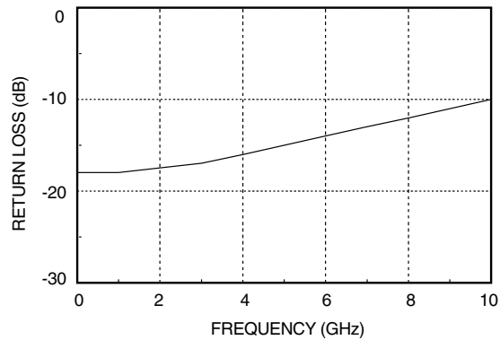
Return Loss
