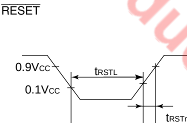
Figure 81 Reset Timing
