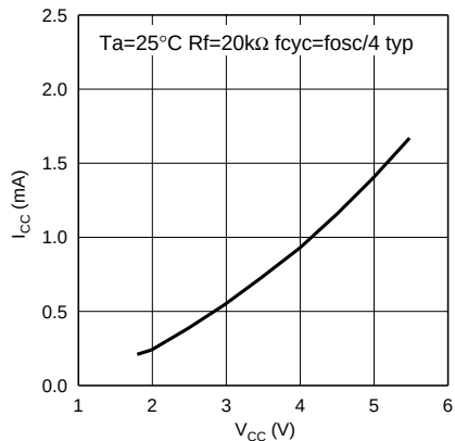
(b) I_{CC} vs. V_{CC} characteristic (resistance oscillation)
