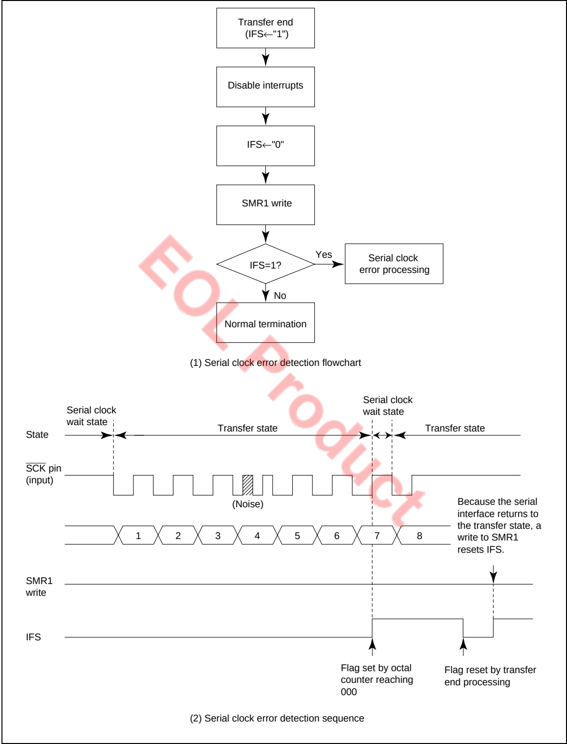
Figure 55 Example of Serial Clock Error Detection
