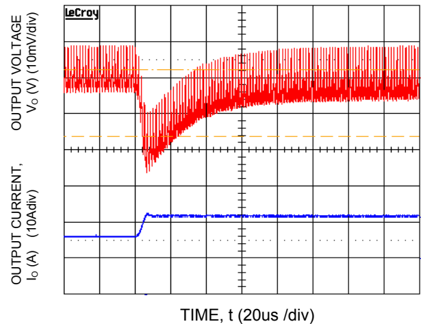
Fig-42. Transient Response to Dynamic Load Change from 50% to 100% at 12Vin, Cout= 1x47μF+3x330μF, CTune=10nF & RTune=220ohms
