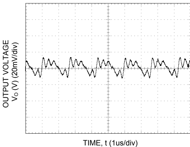
Fig-41. Typical output ripple and noise (CO=22μF ceramic, VIN = 12V, I o = I o,max ).
