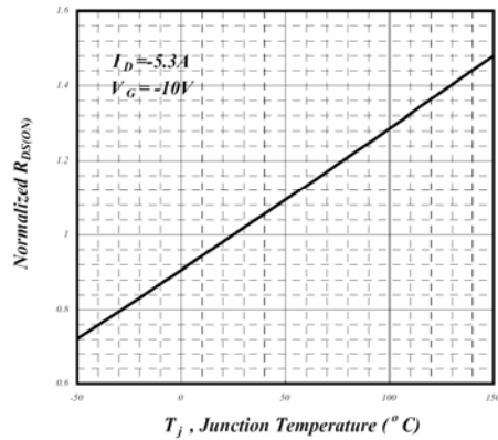
Fig 4. Normalized On-Resistance v.s. Junction Temperature
