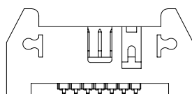
STYLE B 2 X 7
