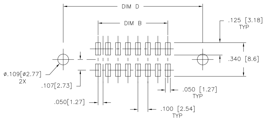
RECOMMENDED P.C. BOARD PAD LAYOUT
