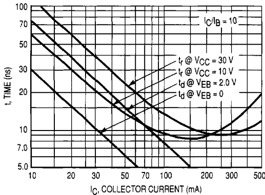
Figure 5. Turn-On Time
