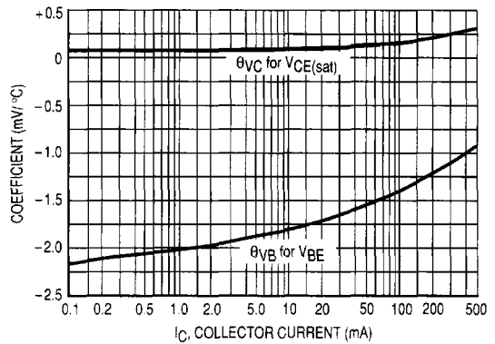
Figure 18. Temperature Coefficients
