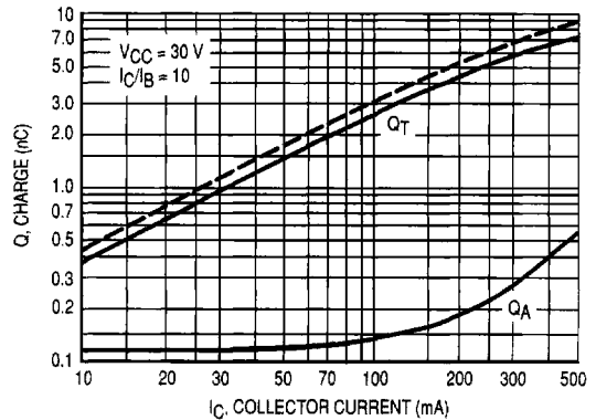
Figure 4. Charge Data
