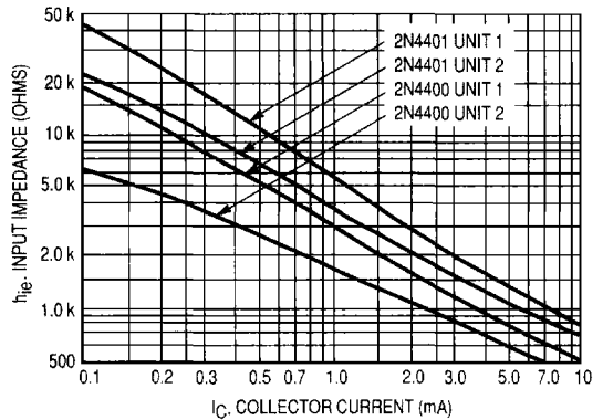
Figure 12. Input Impedance
