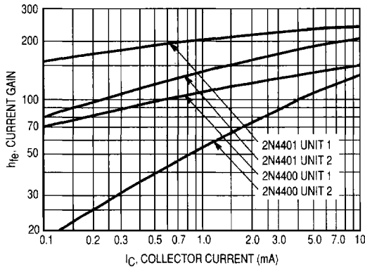
Figure 11. Current Gain
