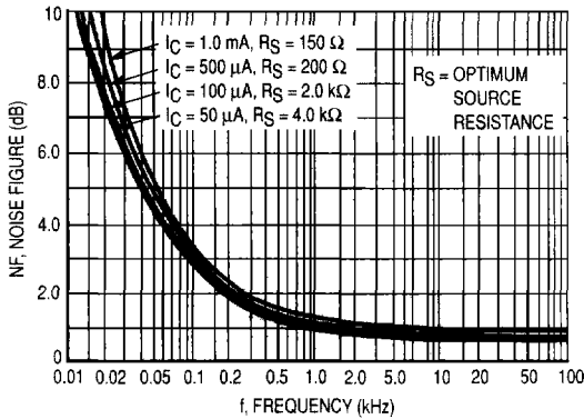
Figure 9. Frequency Effects
