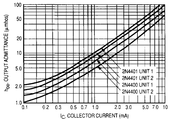
Figure 14. Output Admittance
