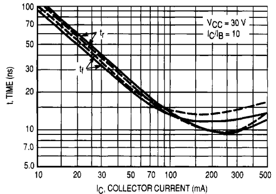
Figure 6. Rise and Fall Times
