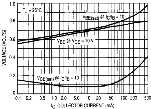
Figure 17. "On" Voltages
