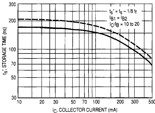
Figure 7. Storage Time
