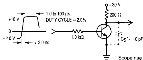
Figure 1. Turn–On Time
