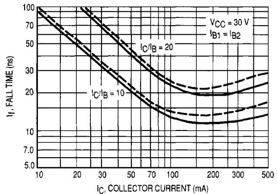
Figure 8. Fall Time
