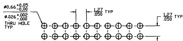
SUGGESTED PCB LAYOUT
