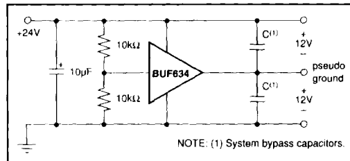
FIGURE 5. Pseudo-Ground Driver.
