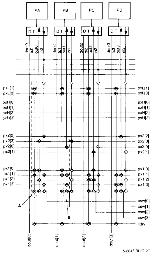
Figure 21. PIC Detail
