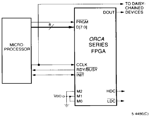
Figure 38. Synchronous Peripheral Configuration Schematic
