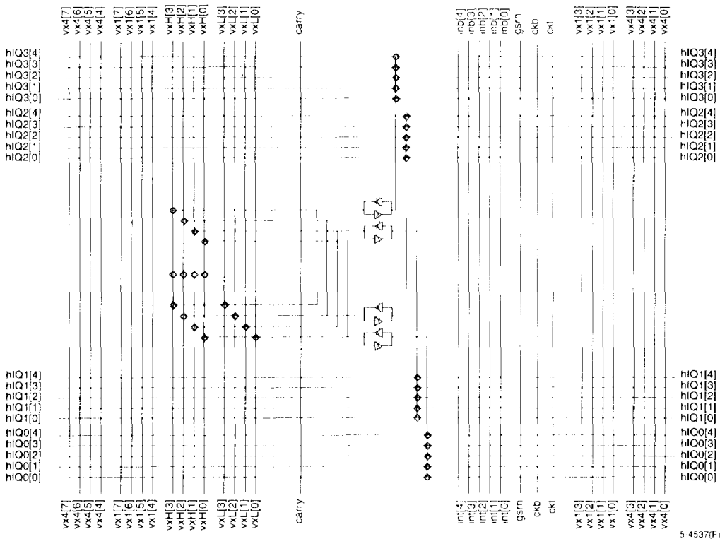
Figure 23. hIQ Block Detail
