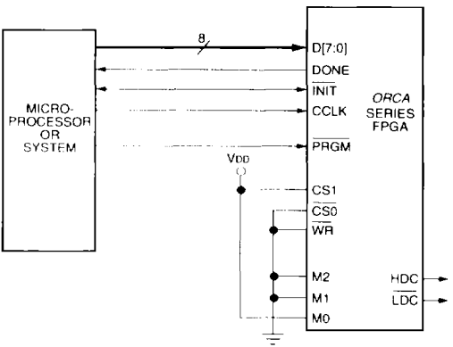
Figure 40. Slave Parallel Configuration Schematic
