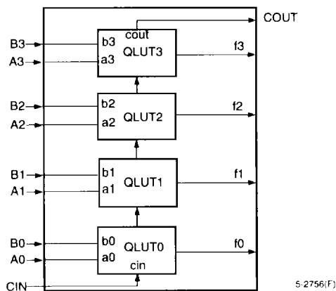
Figure 9. Ripple Mode
