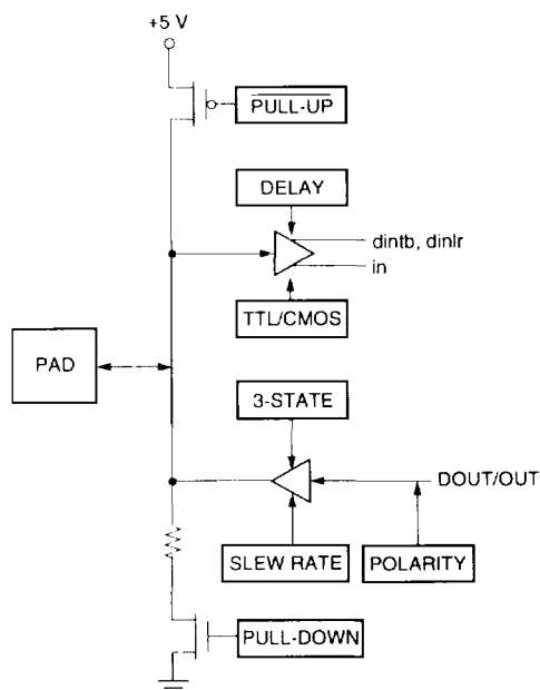
Figure 18. Simplified Diagram of Programmable I/O Cell
