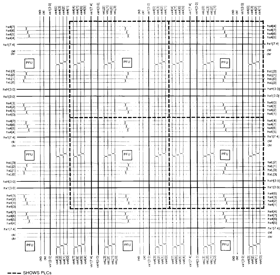
Figure 16. Multiple PLC View of Inter-PLC Routing
