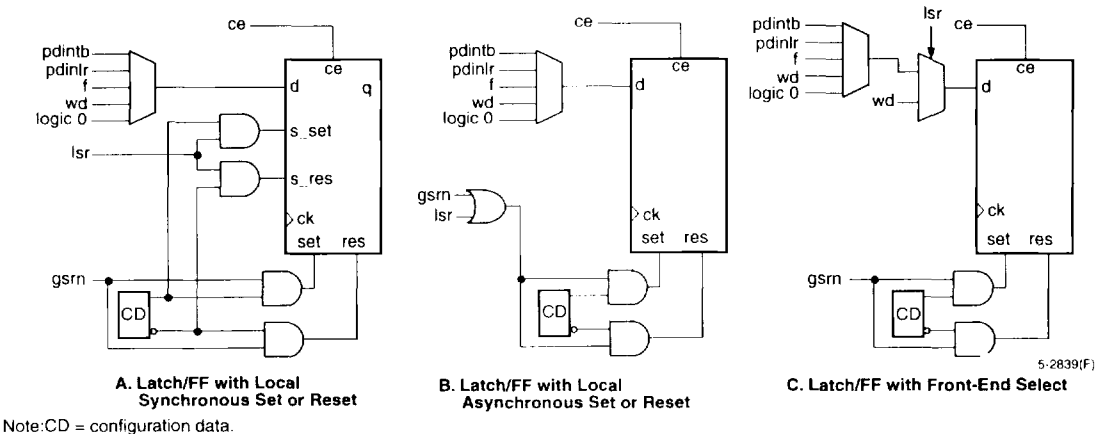
Figure 12. Latch/FF Set/Reset Configurations
