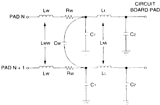
Figure 48. Package Parasitics
