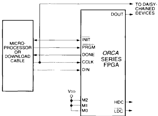
Figure 39. Slave Serial Configuration Schematic
