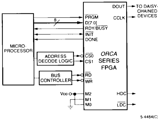
Figure 37. Asynchronous Peripheral Configuration Schematic
