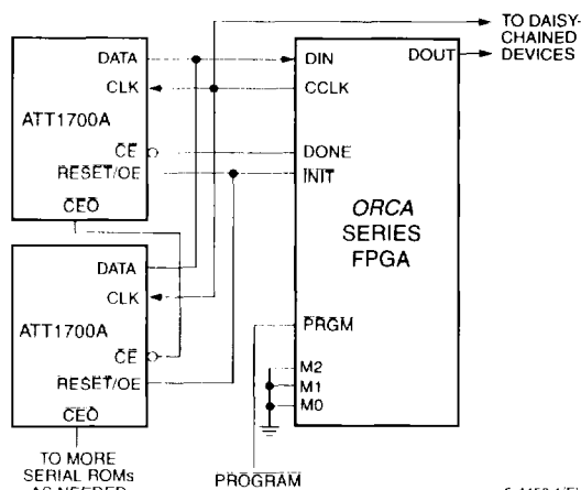
Figure 36. Master Serial Configuration Schematic
