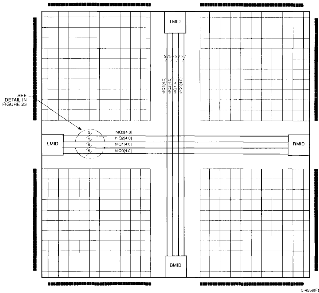
Figure 22. Interquad Routing
