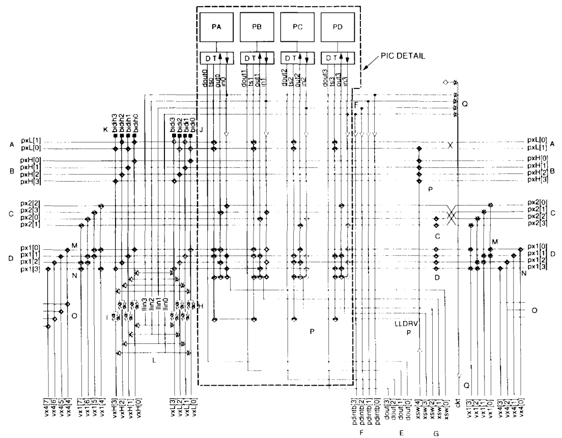
Figure 20. PIC Architecture
