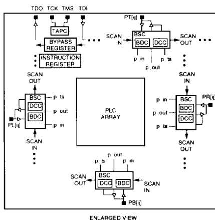
ENLARGED VIEW
