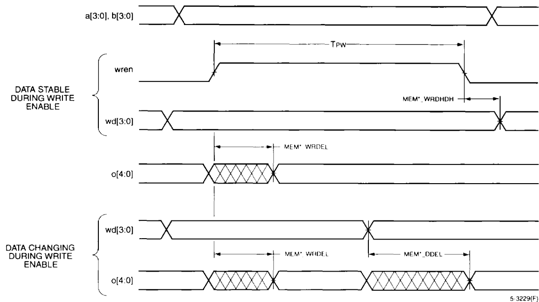
Figure 52. Read During Write
