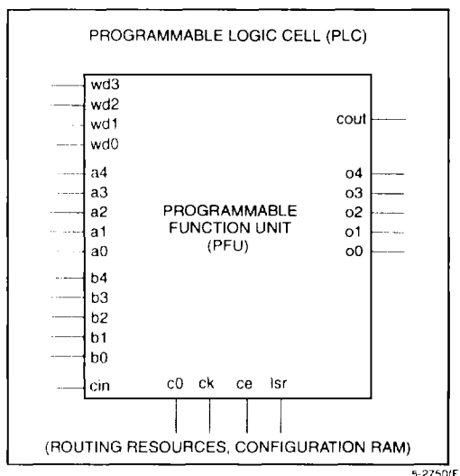
Figure 2. PFU Ports
