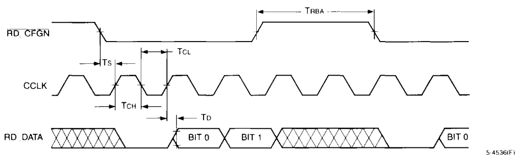
Figure 61. Readback Timing Diagram
