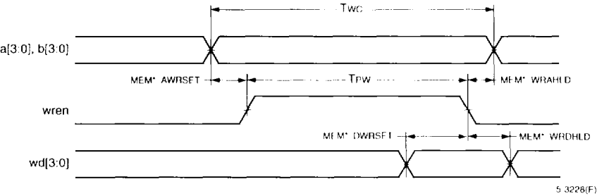
Figure 51. Write Operation
