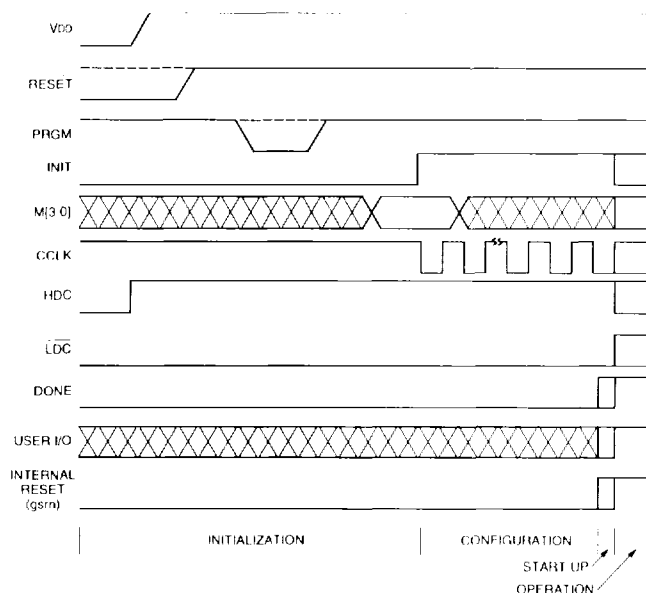
Figure 31. Initialization/Configuration/Start-Up Waveforms
