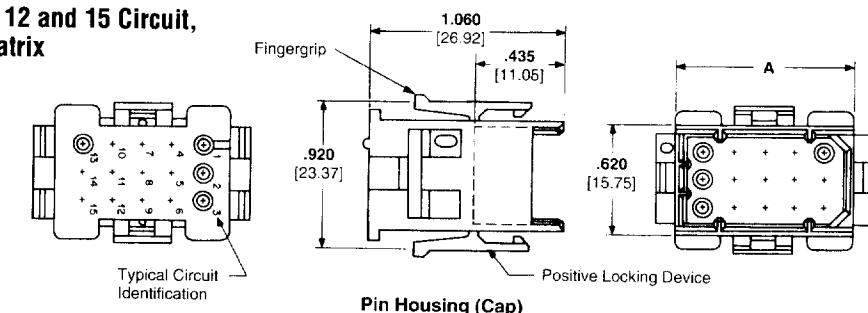
Pin Housing (Cap)
