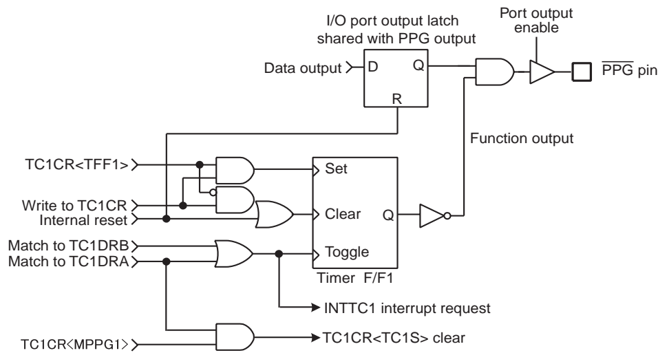
Figure 8-7 \overline{PPG} Output
