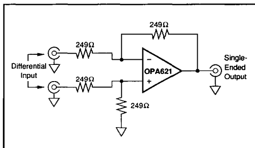
FIGURE 11. Unity Gain Difference Amplifier.
