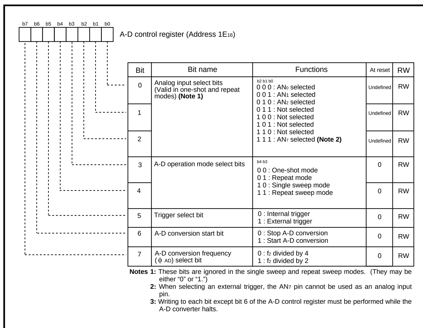
Fig. 20.4.7 Structure of A-D control register
