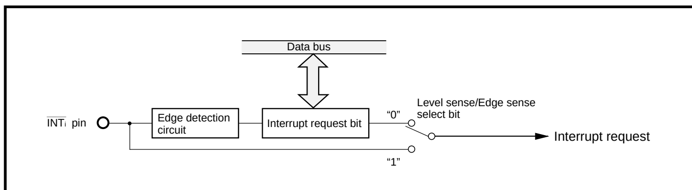
Fig. 4.10.3 Circuit of \overline{\text{INT}}_i Interrupt
