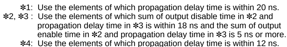
Fig. 17.1.11 Example for using bus buffer (1)
