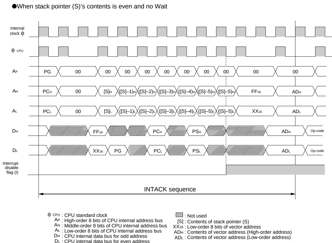
Fig. 4.7.2 INTACK sequence timing (at minimum)
