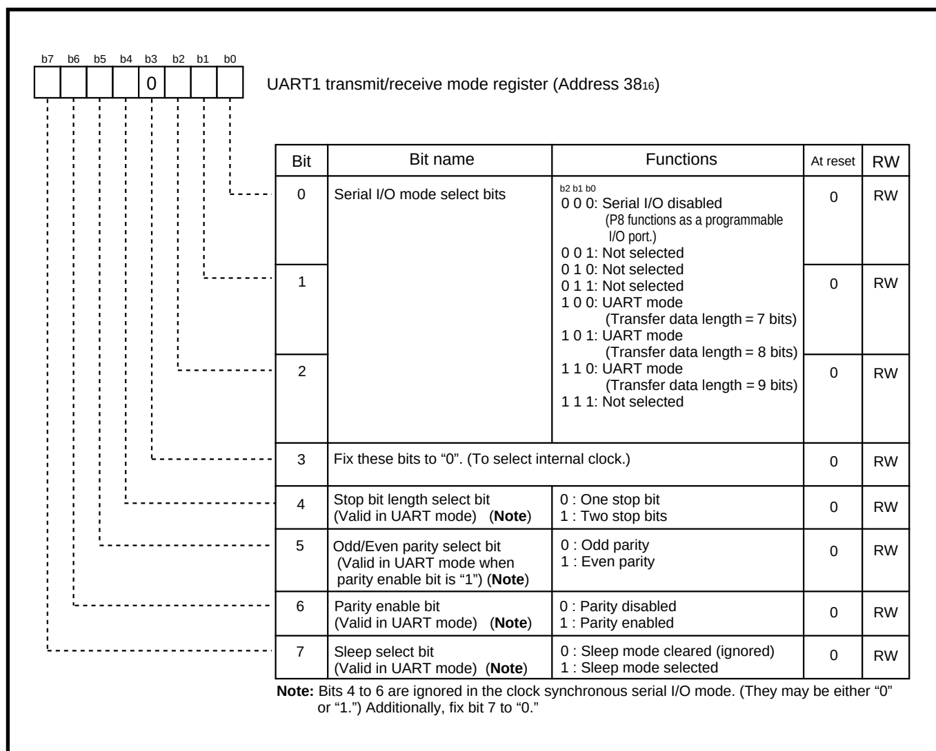
Fig. 20.4.4 Structure of UART1 transmit/receive mode register
