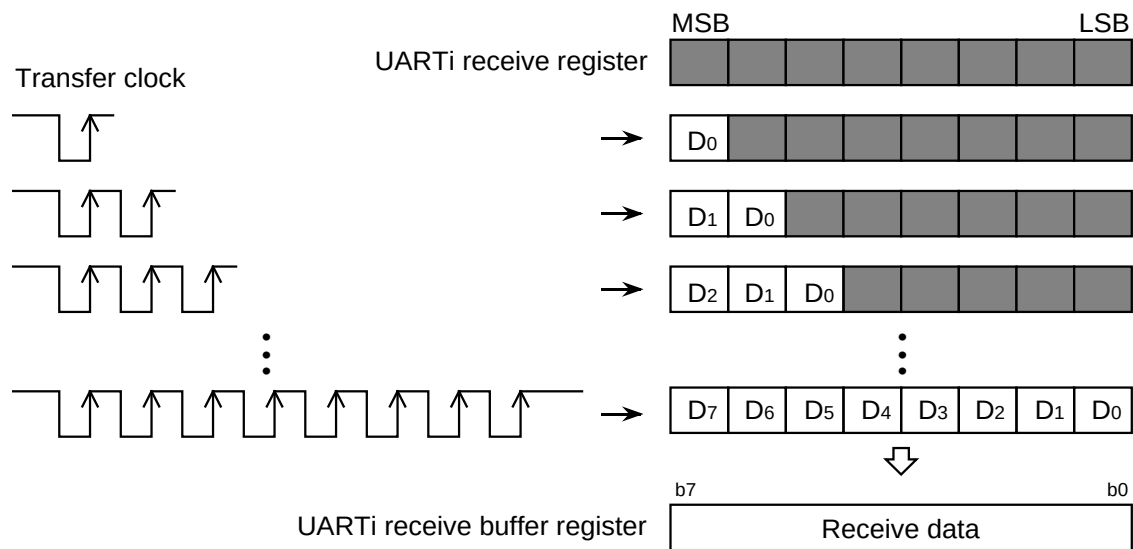
Fig. 7.3.10 Receive operation
