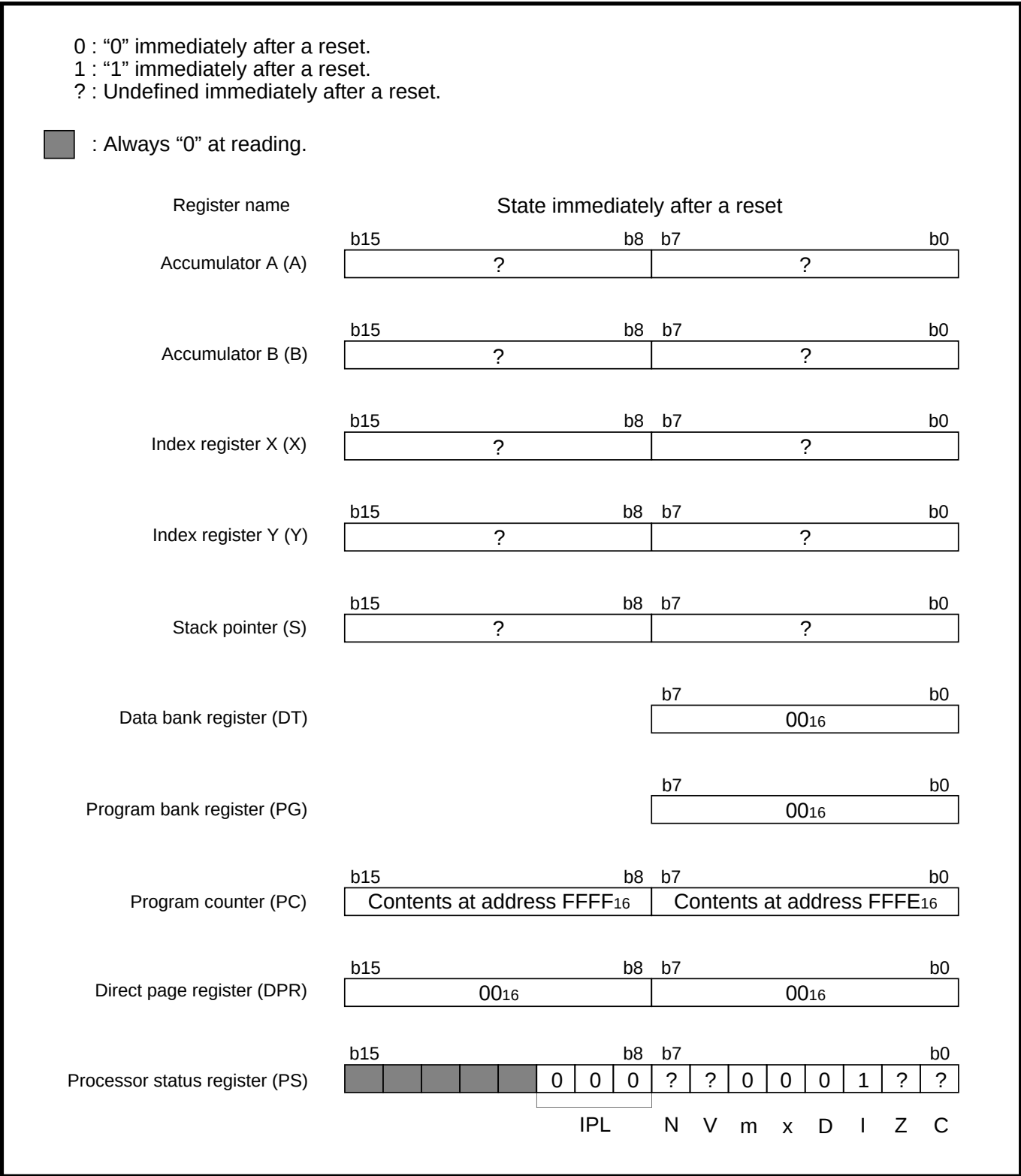
Fig. 13.1.2 State of CPU registers immediately after reset
