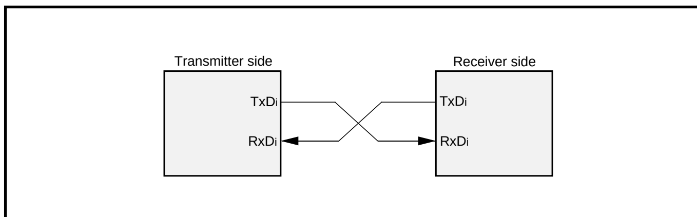
Fig. 7.4.10 Connection example
