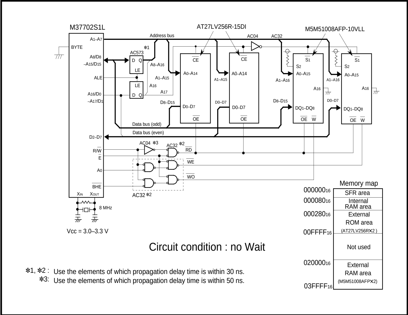
Fig. 18.6.7 Memory expansion example on maximum model
