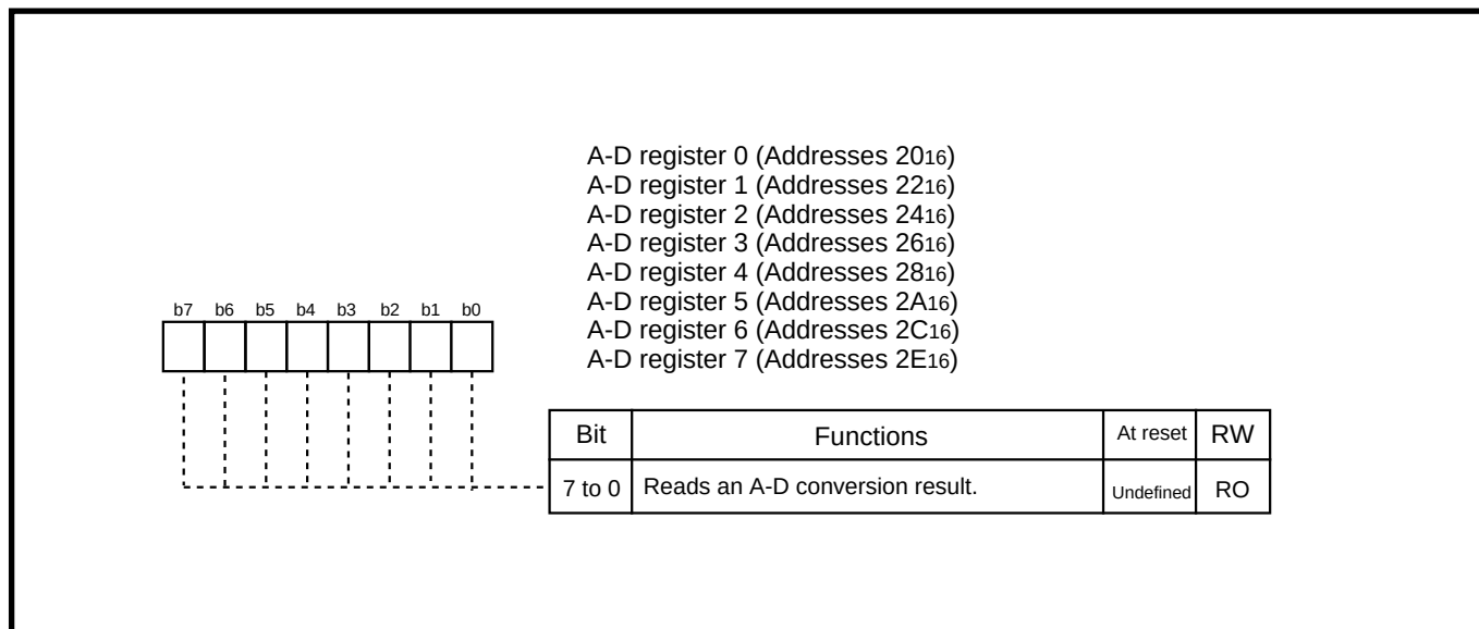
Fig. 8.2.4 Structure of A-D register i
