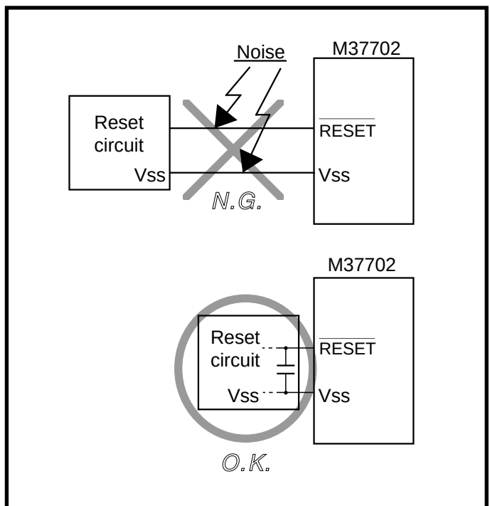
Fig. 10 Wiring of \overline{\text{RESET}} pin
