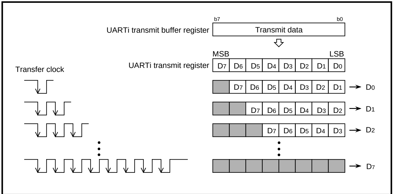
Fig. 7.3.4 Transmit operation
