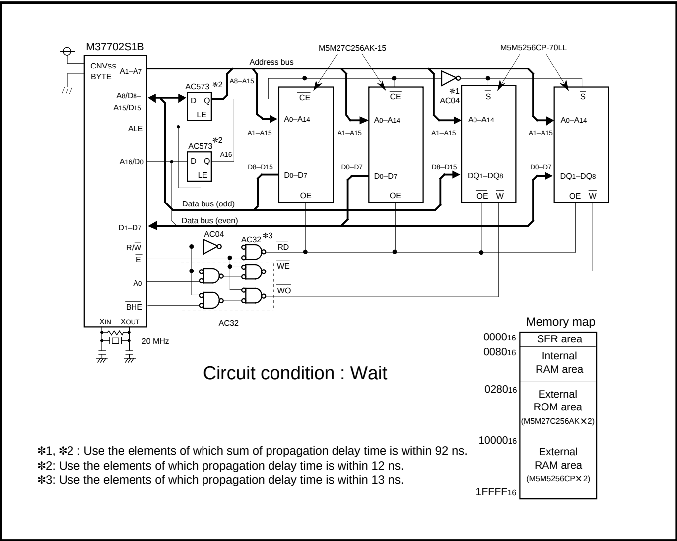
Fig. 17.1.19 Example of ROM and SRAM expansion (maximum model)
