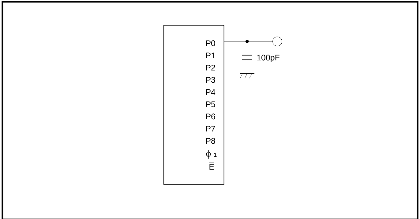
Fig. 15.10.1 Testing circuit for ports P0 to P8, \phi_1 , and \overline{E}
