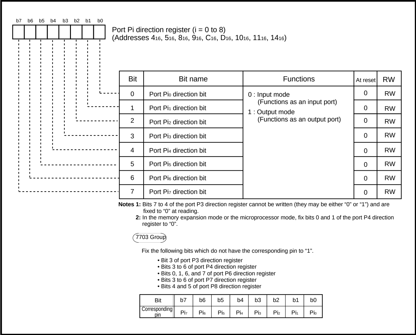
Fig. 3.1.2 Structure of port P_i ( i = 0 to 8) direction register
