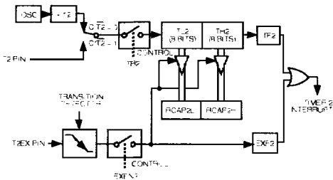
Figure 7. Timer 2 in Capture Mode.
