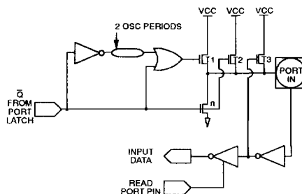
Figure 4. I/O Buffers in the 80C52 (Ports 1, 2, 3).
