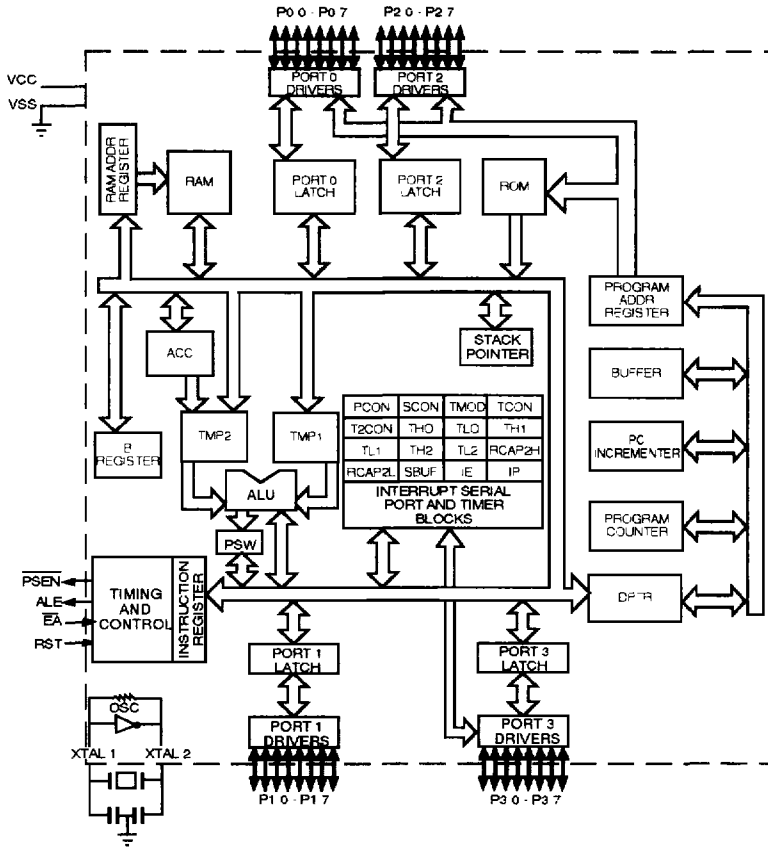
Figure 1. Block Diagram
