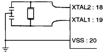
Figure 5. Crystal Oscillator.
