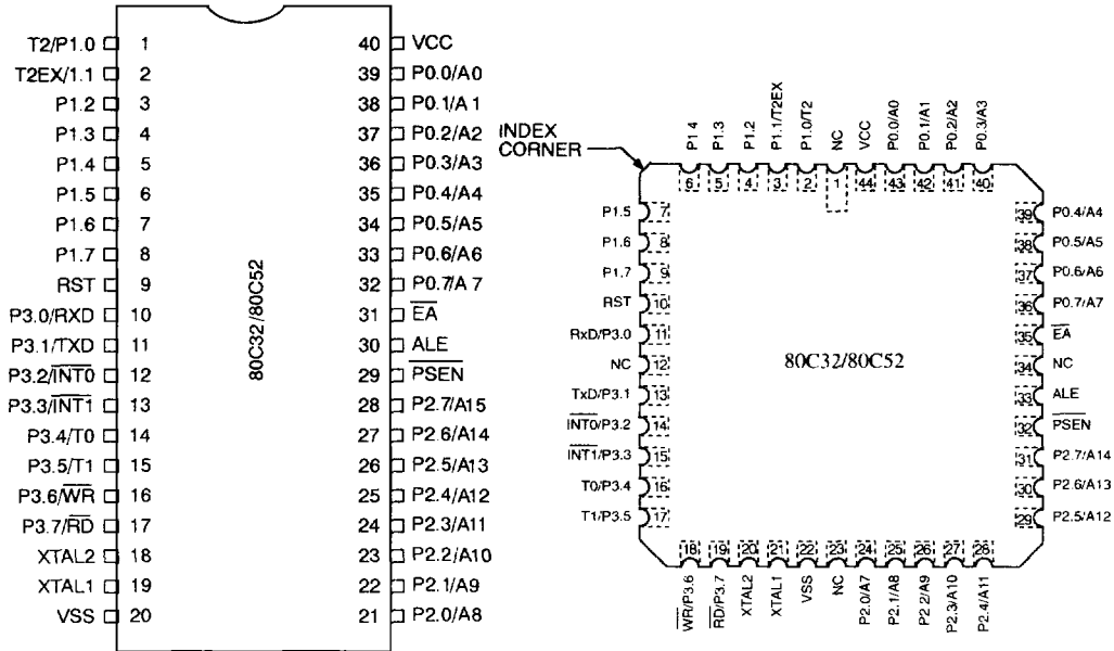
Figure 2. Pin Configuration
