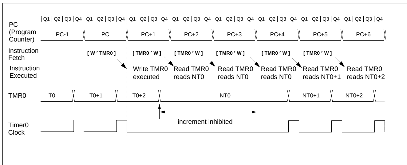
FIGURE 11-3 TIMER0 TIMING: INTERNAL CLOCK/NO PRESCALE
