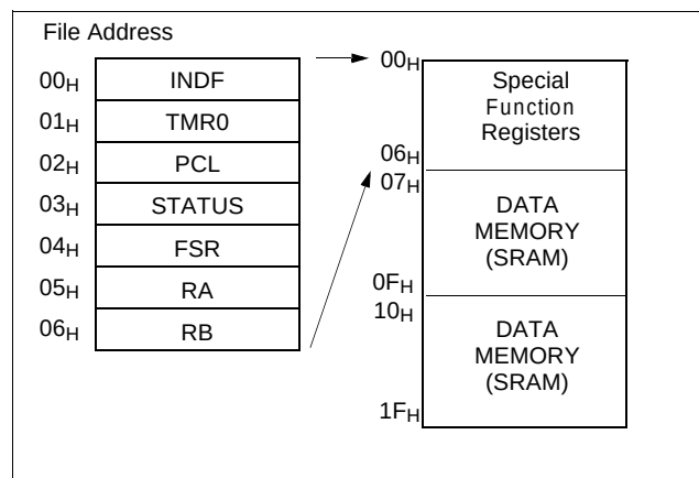
FIGURE 9-3 HMS77C100XA DATA MEMORY MAP
