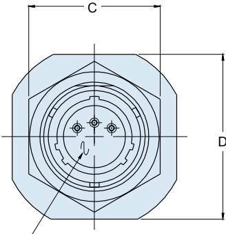
Insert Arrangement, per MIL-C-38999, Series I
