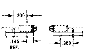
TWO PRINTED CIRCUIT VARIANTS 001, 004
