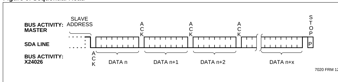
Figure 9. Sequential Read
