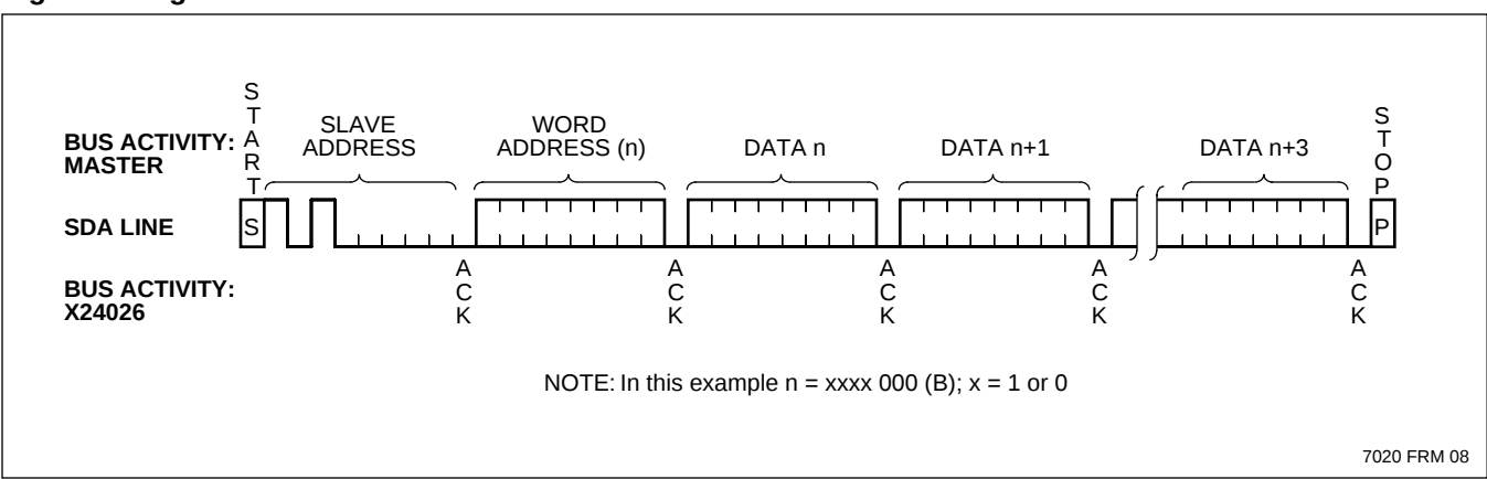
Figure 6. Page Write
