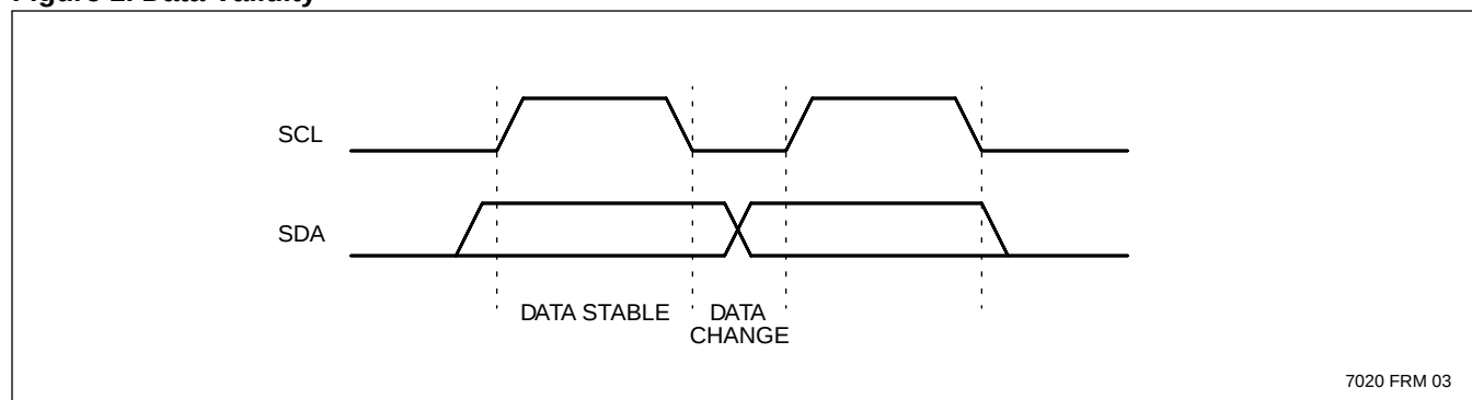
Figure 1. Data Validity
