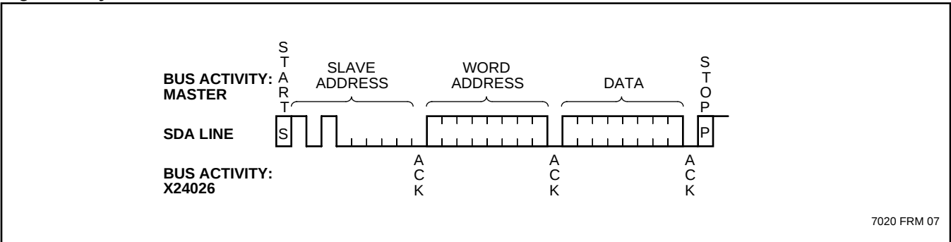
Figure 5. Byte Write
