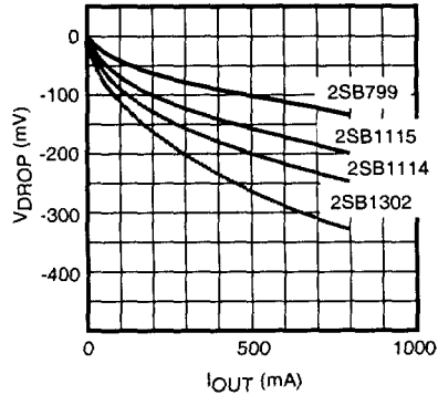
DROPOUT VOLTAGE vs. OUTPUT VOLTAGE
