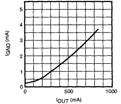
GROUND CURRENT vs. OUTPUT VOLTAGE
