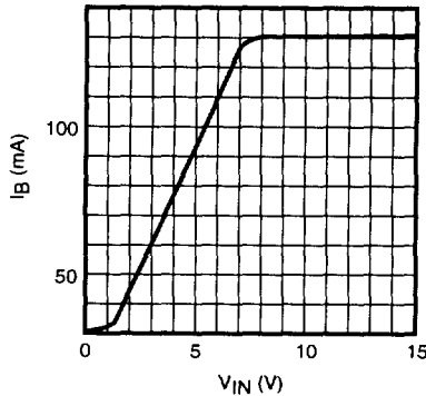
BASE CURRENT DRIVE vs. INPUT VOLTAGE
