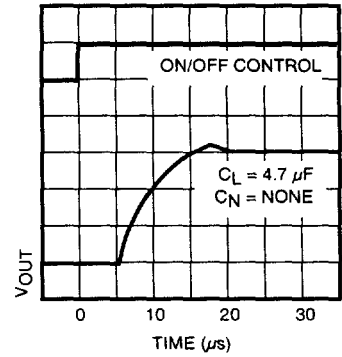
ON/OFF STEP RESPONSE
