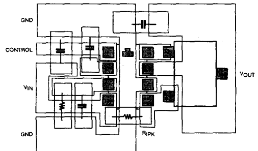
SOT23L-8 BOARD LAYOUT
