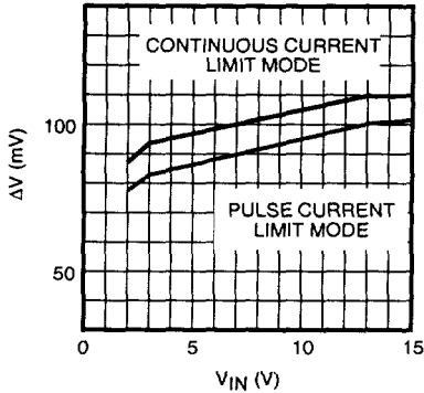
CURRENT LIMIT DETECTOR VOLTAGE vs. INPUT VOLTAGE
