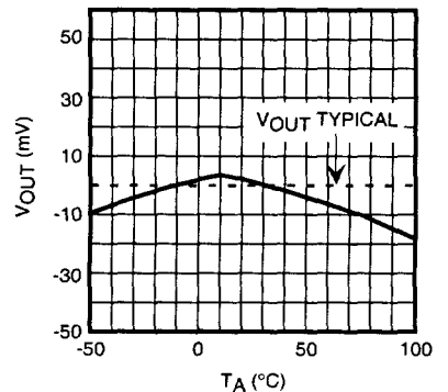
OUTPUT VOLTAGE VARIATION vs. TEMPERATURE
