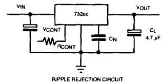
RIPPLE REJECTION CIRCUIT
