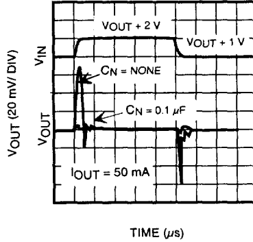
LINE CURRENT STEP RESPONSE
