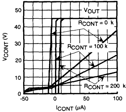
CONTROL PIN VOLTAGE vs. CONTROL CURRENT
