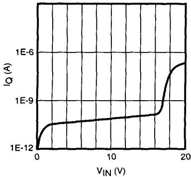
QUIESCENT CURRENT vs. INPUT VOLTAGE (OFF MODE)
