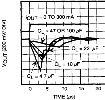
LOAD CURRENT STEP RESPONSE
