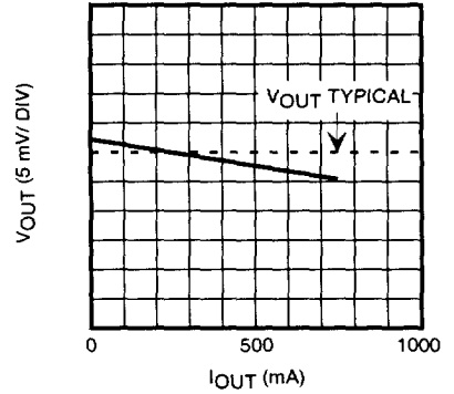
LOAD REGULATION
