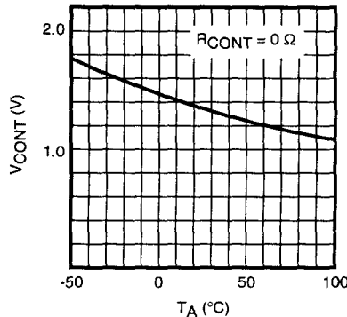
CONTROL VOLTAGE (OUTPUT ON POINT) vs. TEMPERATURE
