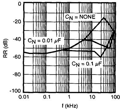
RIPPLE REJECTION
