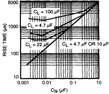
ON/OFF TRANSIENT
