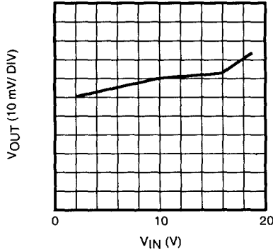
LINE REGULATION 2
