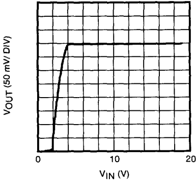
LINE REGULATION 1
