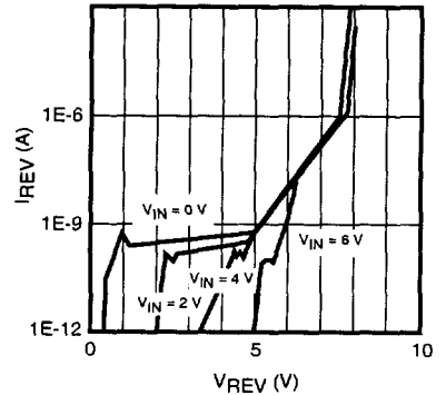
REVERSE BIAS CURRENT (V_IN = 0 TO 6 V)
