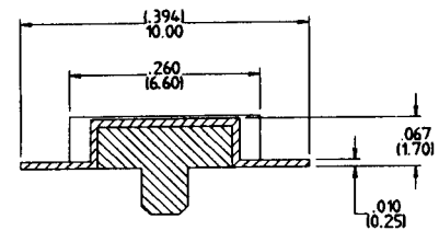
SECTION Y-Y
