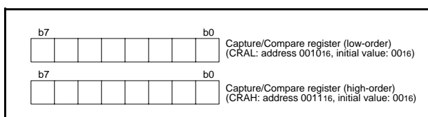
Fig 29. Structure of capture/compare register
