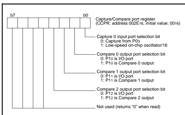
Fig 32. Structure of capture/compare port register
