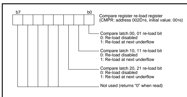
Fig 31. Structure of compare register re-load register
