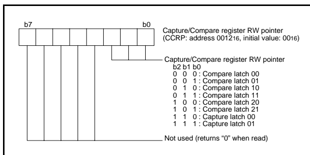
Fig 30. Structure of capture/compare register RW pointer
