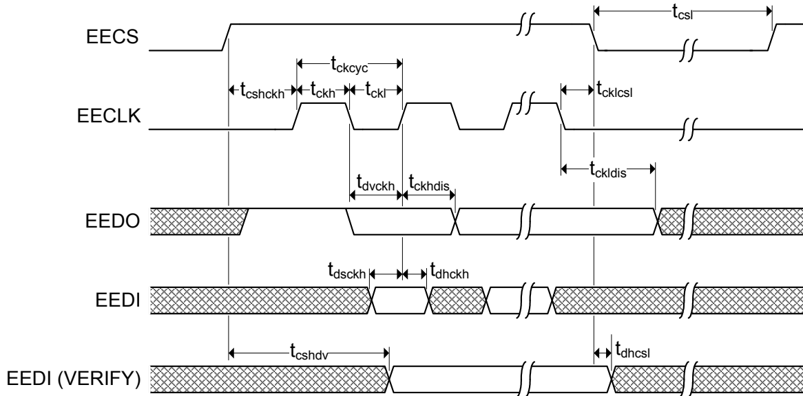
Figure 15.10 Microwire Timing
