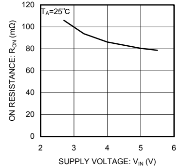
Fig.12 On-resistance
