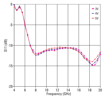
Figure 15. Typical Input Return Loss over Vdd (supply voltage)
