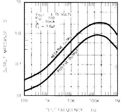
FIGURE 12. OUTPUT IMPEDANCE
