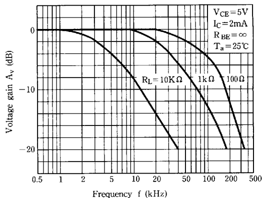
Fig.12 Frequency Response
