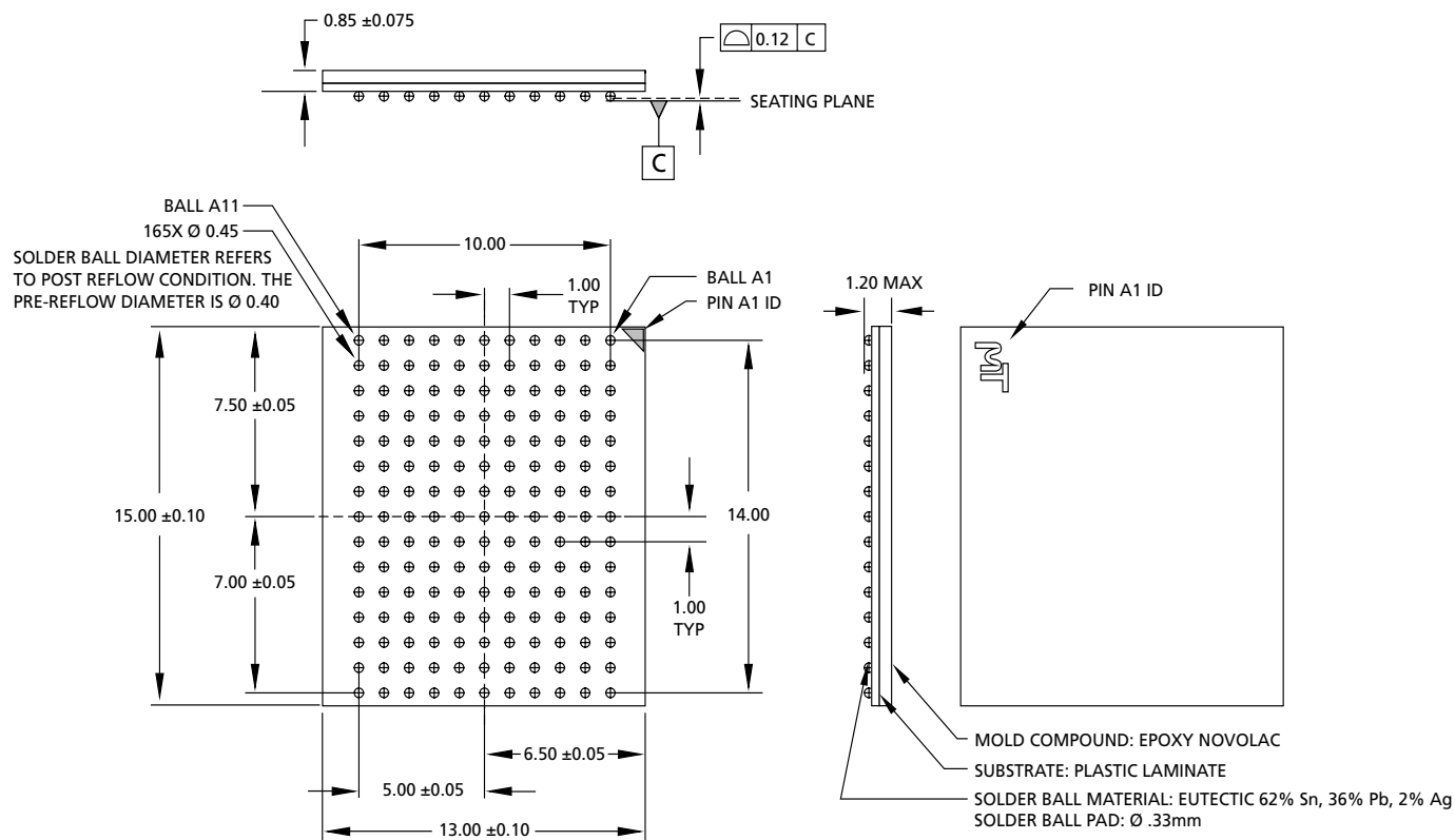
Figure 21: 165-Ball FBGA
