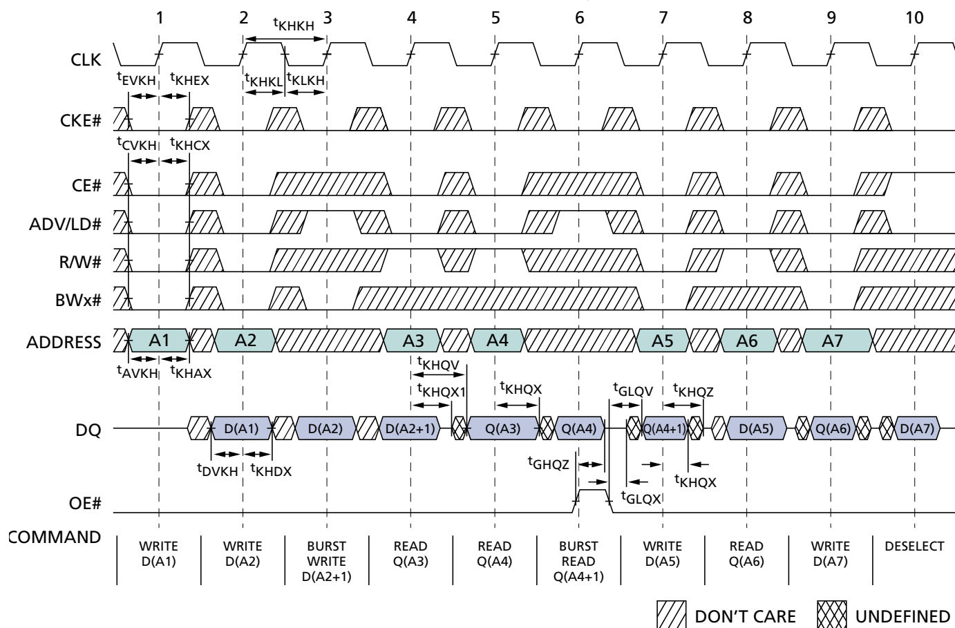
Figure 8: READ/WRITE Timing
