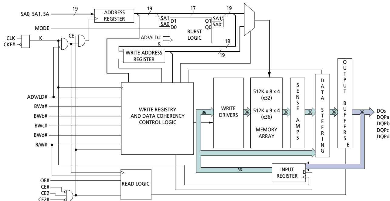
Figure 4: Functional Block Diagram 512K x 32/36
