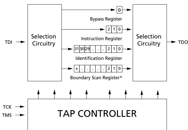
Figure 16: TAP Controller Block Diagram
